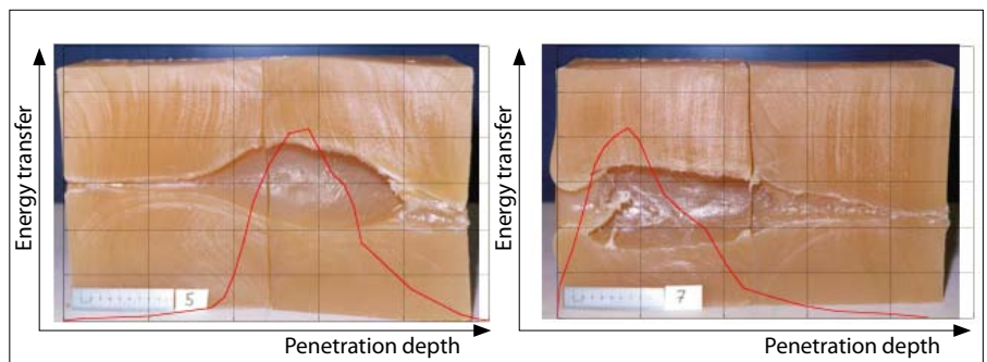
Figure 3.19 Soap blocks showing comparison between ballistic profiles of FMJ and SJ bullets – the transfer of kinetic energy occurs far sooner with the SJ bullet.
